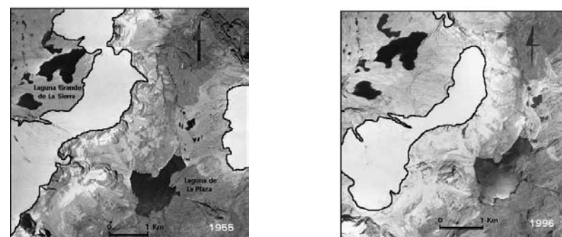
Figure 2: Retreating glaciers in El Cocuy in the Sierra Nevada comparing 1955 with 1996
