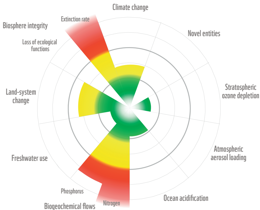
Figure 8: Planetary Boundaries
