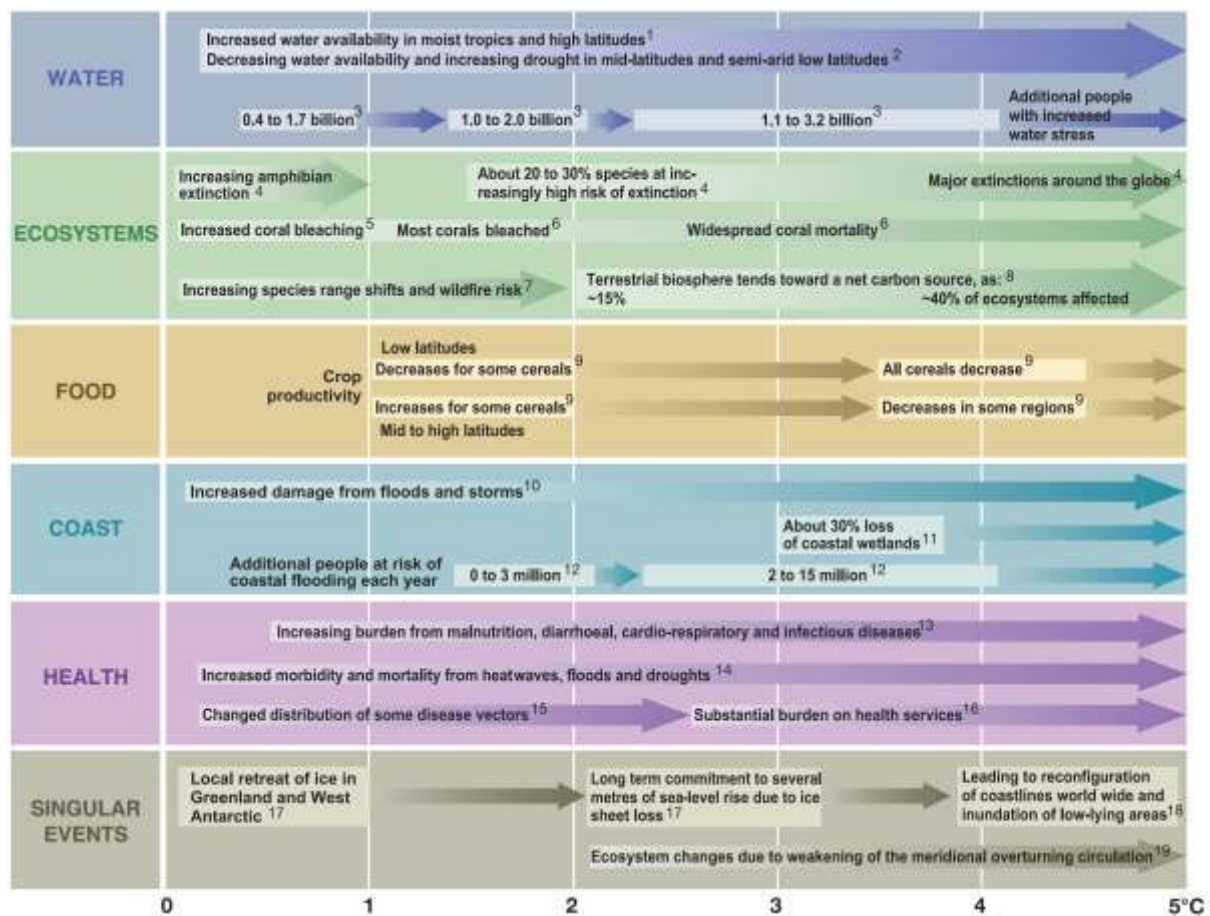
Figure 1. Examples of impacts associated with global average temperature change in the 21st century (note that x axis is relative to temperature increase in 1980-1999, which is 0.5°C above pre-industrial). From IPCC 4AR (WGII, Table TS.3).
