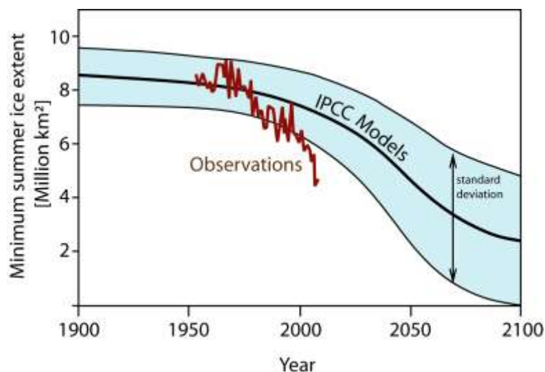
Figure 3. Observations (1953-2008) and predictions (mean and range of IPCC models driven with the A1B scenario) of arctic minimum summer sea ice extent (courtesy of D. Notz, Max Planck Institute for Meteorology).
